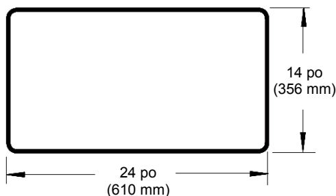
Figure 1. Protection de plancher minimum.
