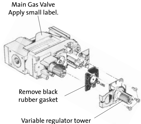
Figure 27. Regulator assembly.
