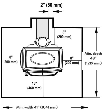
Fig. 8b. F 445 Hearth Dimensions Canada.
