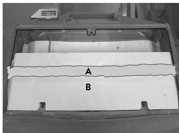
Fig. 22. Insulation gasket (A) and Insulation panel (B).
