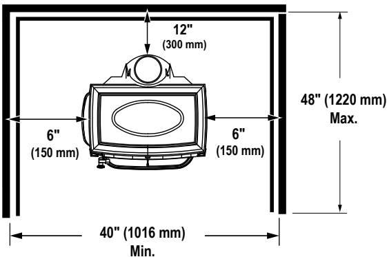
Fig. 10. Alcove protected wall clearances are designated between the stove surfaces and the combustible wall surface.
