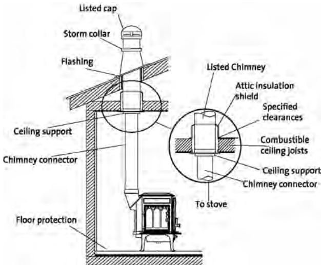
Fig. 7. Prefabricated chimney components.
