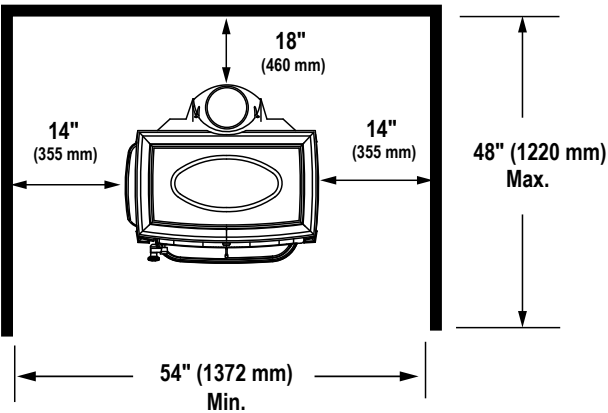
Fig. 9. Alcove unprotected wall clearances.
